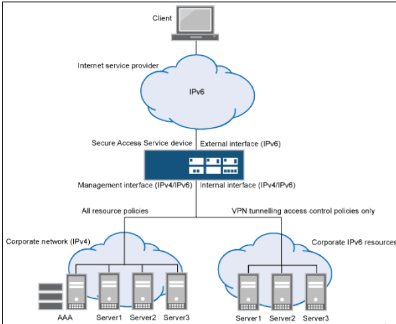
Dual Stack Endpoint Access Over ISP IPv6 Network:
